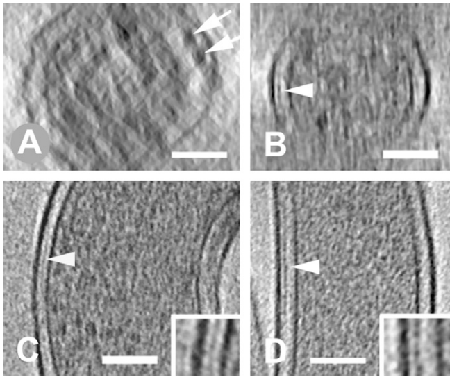
Fig. 1. Widening of the periplasmic space in the presence of flagellar filaments, and position of the peptidoglycan layer. (A) Cross-section of wild-type cell (WT-4) with widened periplasmic space, accommodating two flagellar filaments on the upper right (arrows). (B) Cross-section of aflagellate mutant cell (Afla-1) showing uniform periplasmic space and a peptidoglycan layer (arrowhead). The membranes at the top and bottom are poorly defined due to the tomographic missing wedge. (C) Peptidoglycan layer (arrowhead, inset) in longitudinal slice of another wild-type cell. (D) Peptidoglycan layer (arrowhead, inset) in aflagellate mutant; longitudinal slice represented by cross-section in (B). Tomographic slices 1.8 nm (A and B) and 9 nm (C and D) thick; scale bars = 100 nm.
