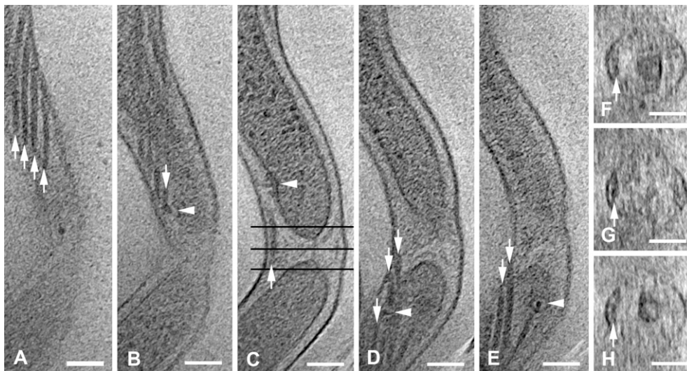
Fig. 2. Overlap of periplasmic flagellar filaments at the cell constriction site (cell WT-11). (A) Four-flagellar filaments (arrows). (B) Basal body ring (arrowhead), giving rise to flagellar filament (arrow); depth at 27 nm below (A). (C) Flagellar filament (arrow) passing through cell constriction site; side view of the second basal body ring (arrowhead); depth 63 nm below (B). Black lines indicate position of cross-sections shown in (F), (G), and (H). (D) Crossing of the two flagellar filaments (upper arrows); basal body ring (arrowhead) giving rise to flagellar filament (lower arrow); depth 59 nm below (C). (E) Continuation of the two flagellar filaments that crossed the constriction site (arrows); second basal body ring (arrowhead); depth 13 nm below (D). (F) Cross-section at tip of upper cytoplasmic cylinder (black line in (C)), showing two closely apposed flagellar filaments (arrow); separation between filaments, and continuity of the outer membrane are poorly defined due to the tomographic missing wedge. (G) Cross-section midway between the cytoplasmic cylinders, with continuation of flagellar filaments (arrow). (H) Cross-section at the tip of the lower cytoplasmic cylinder, with continuation of flagellar filaments (arrow). Tomographic slices, 1.8 nm thick; scale bars = 100 nm.
