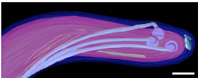
Fig. 4. Surface-rendered model of WT-10 cell end showing three flagellar filaments arising from basal bodies (blue), a periplasmic patella-shaped structure (light blue), a plate-like structure (green), and cytoplasmic filaments (yellow). The outer membrane is dark blue, and the cytoplasmic cylinder is purple. An animation of this surface-rendered model is presented in supplemental material (Movie S1). Scale bar = 100 nm.
