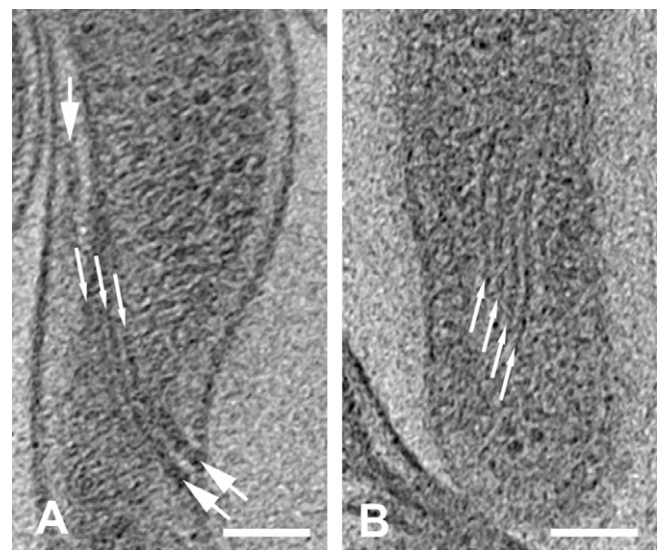
Fig. 5. Cytoplasmic filaments in wild-type and aflagellate strains. (A) Cytoplasmic filaments (thin arrows) and flagellar filaments (arrows) in wild-type cell WT-4. The flagella are parallel and above the cytoplasmic filaments, so only the downward-curving portion is seen in the periplasmic space. (B) Cytoplasmic filaments (thin arrows) in the aflagellate strain (cell Afla-4). Tomographic z-slices, 1.8 nm thick; scale bars = 100 nm.
