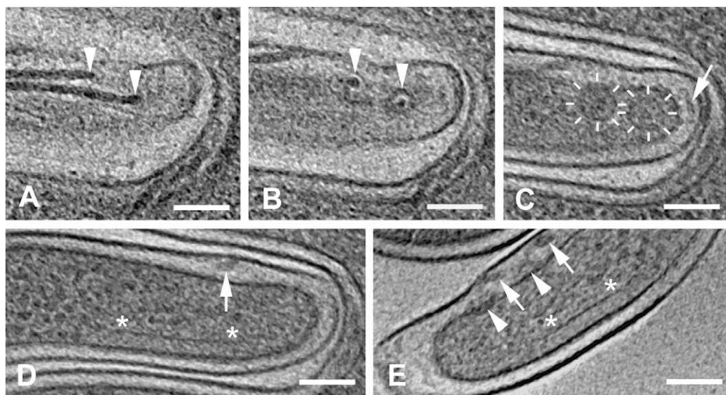
Fig. 3. Flagellar filament basal bodies and profiles of a plate-like structure. (A) Slice at the level of the hooks (arrowheads), attaching the flagellar filaments to the basal bodies. (B) Slice 18 nm below (A), showing upper rings of the flagellar basal bodies (arrowheads). (C) Slice 32 nm below (B) showing the larger lower rings of the flagellar basal bodies (indicated by radial line segments). Also seen in (C) is a cell-end patella-shaped structure (also shown in Fig. 4). (D) Slice 34 nm below (C), showing a flagellar filament (arrow) in a widened periplasmic space, and a profile of a plate-like structure (shown in Fig. 4), the two ends of which are marked (*). (A–D) are from cell WT-10. (E) Side views of basal bodies and hooks from cell WT-8. The periplasmic rings (arrowheads) are below the hooks (barely visible), giving rise to the flagellar filaments (arrows). This cell also has a profile (indicated by * at both ends) of a plate-like structure. Additional membranes from an adjacent cell are seen above and below the cell end of interest in (A–D) (see Figure S2 for a larger field of view). Tomographic slices, 1.8 nm thick; scale bars = 100 nm.
